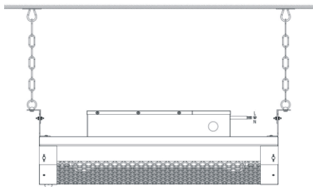
Suspend mount
