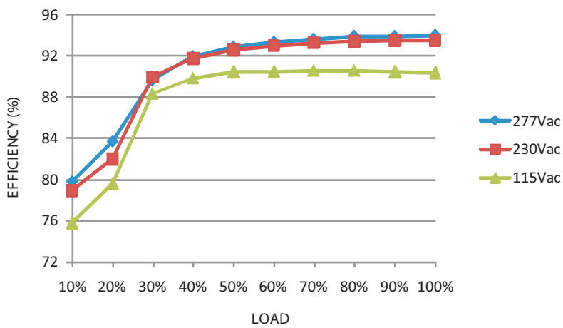
■ EFFICIENCY vs LOAD (48V Model)
