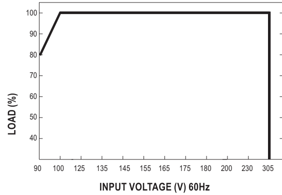
■ Static Characteristics
